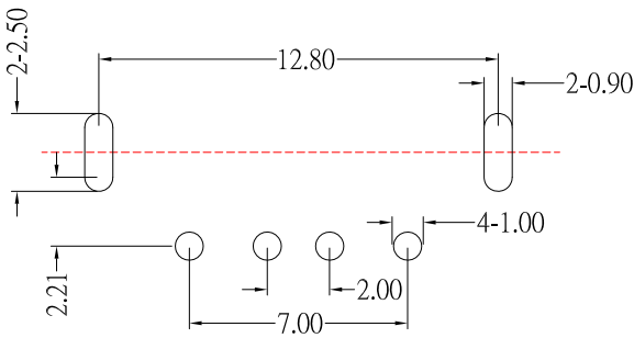
P.C.B LAYOUT MOUNTING PATTERN
